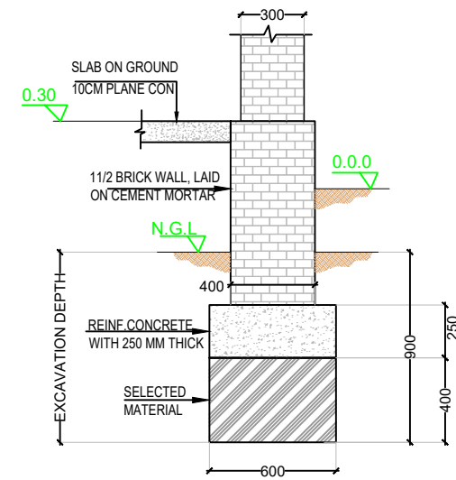
STRIP FOOTING
