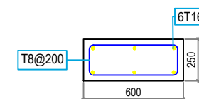
STRIP FOOTING DETAILS
